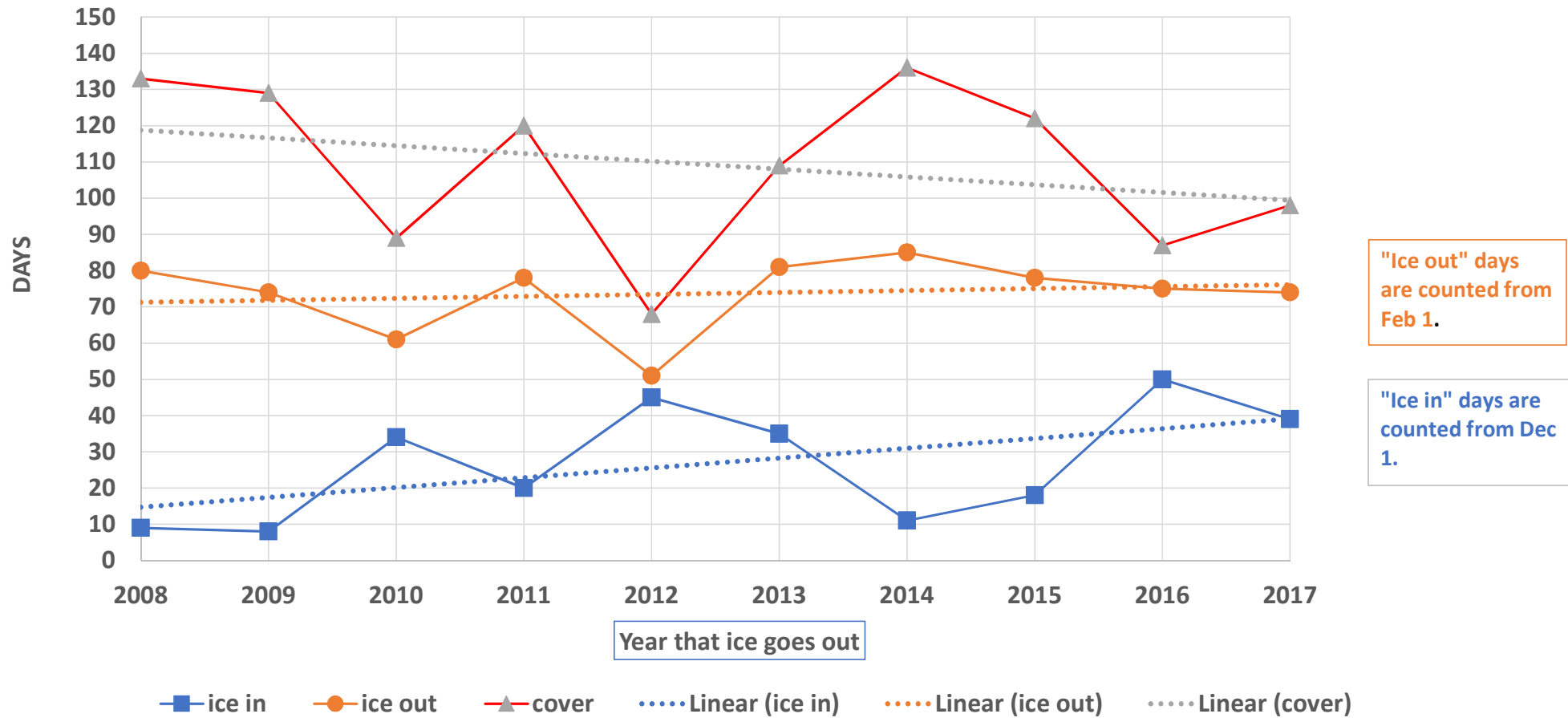
Fig 5 Chandos Ice Cover, 2008-2017 (From Bruels)
